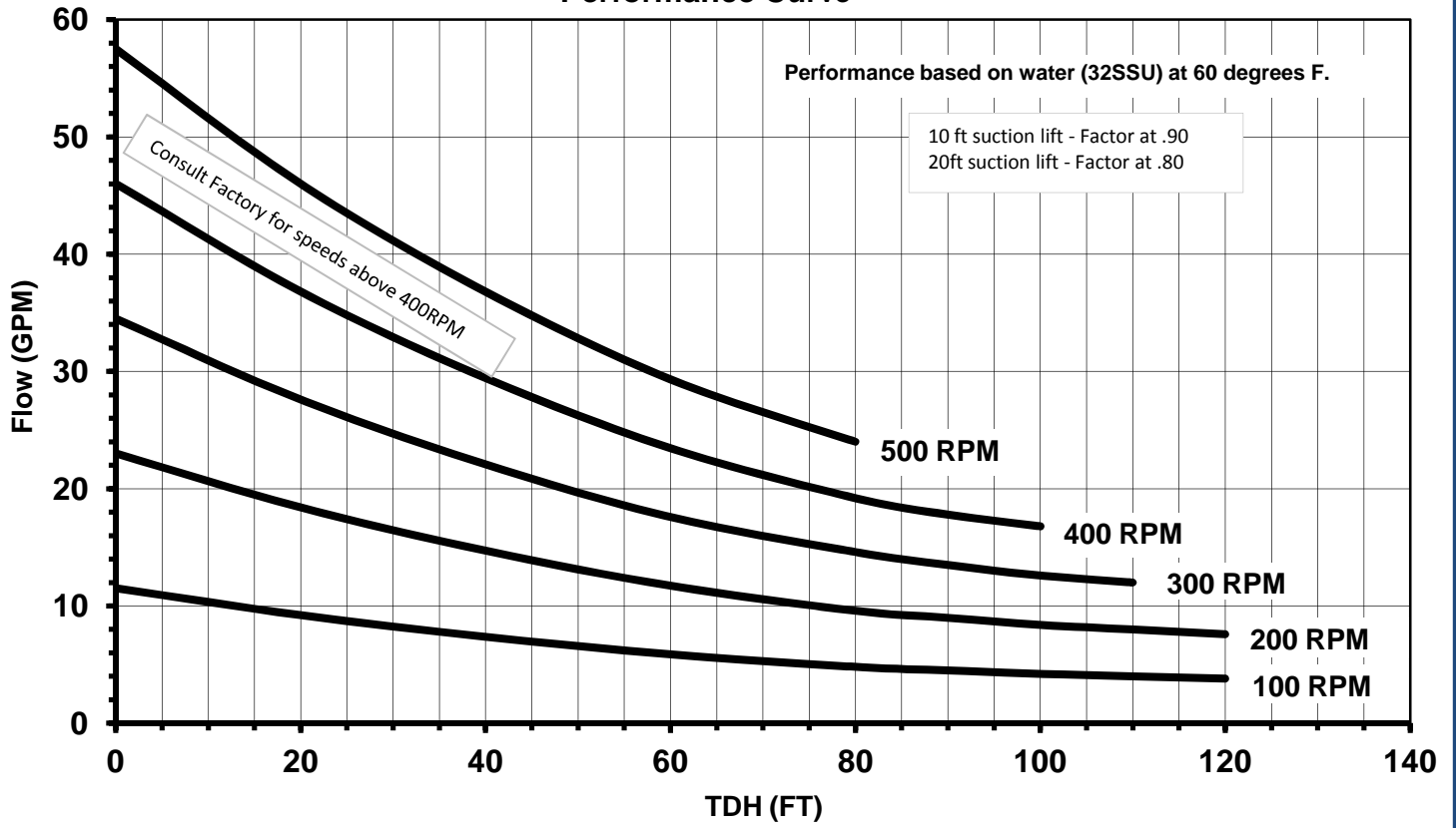
Performance Curve
